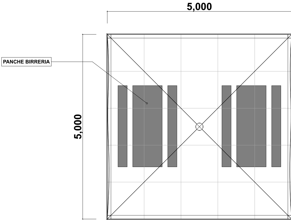
PIANTA GAZEBO 5X5
